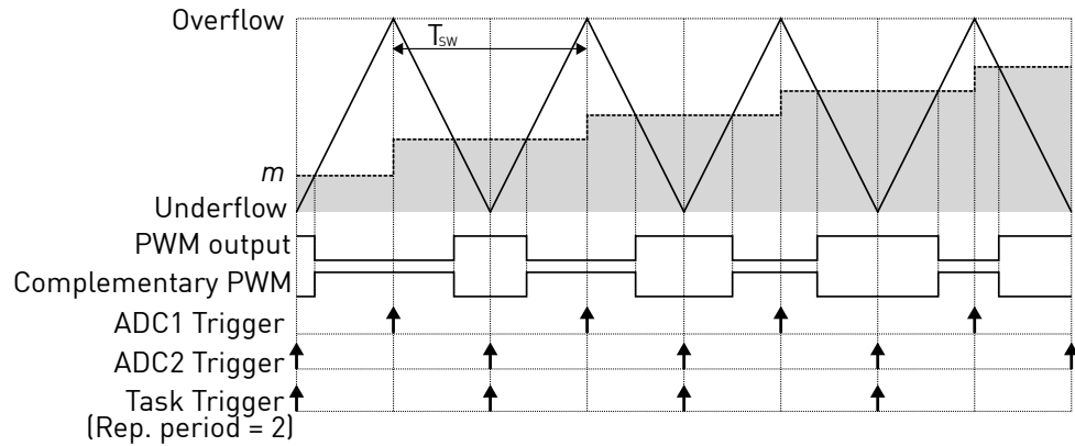
Fig. 2.10: PWM carrier and interrupts for phase-shifted ADC sampling
