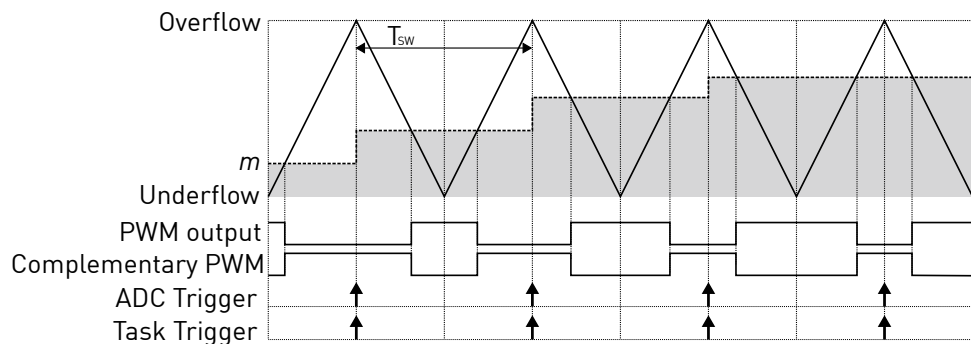
Fig. 4.15: PWM and trigger schemes for symmetric carrier
