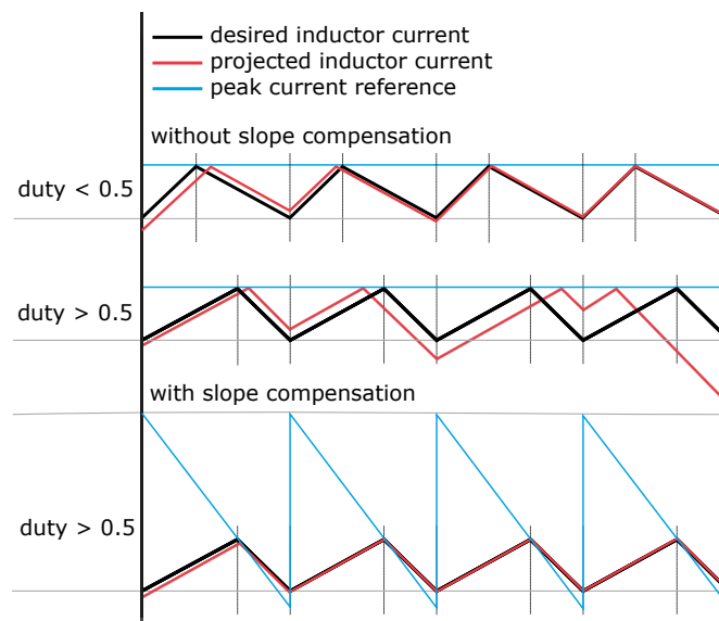
Fig. 4.9: Slope compensation
