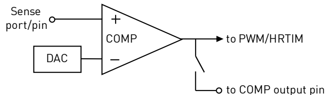
Fig. 3.1: Setup for an analog protection signal.
