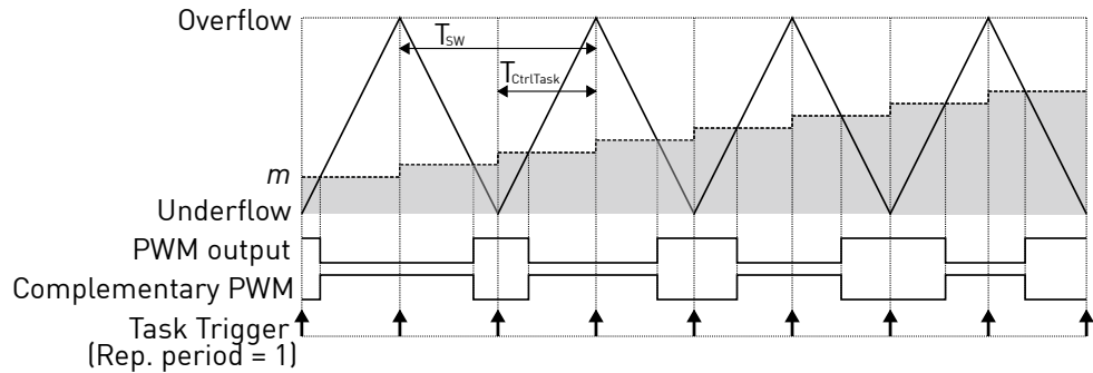
Fig. 2.6: PWM carrier and task interrupts for PWM frequency set to half the control task frequency
