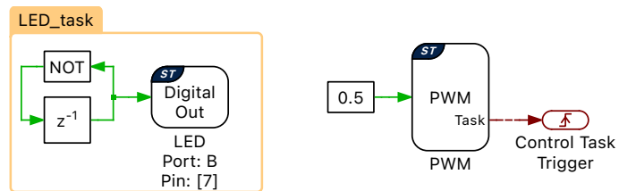
Fig. 2.12: Example of an additional LED task along with a base PWM task
