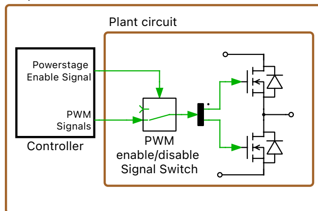
Top-level schematic
