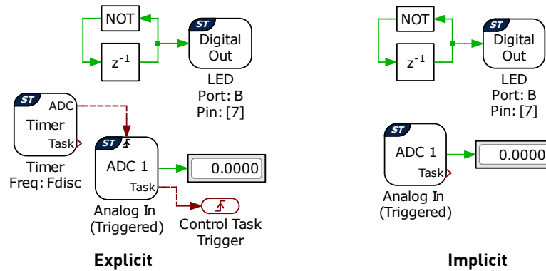
Fig. 2.3: Basic model with control task triggered by ADC
