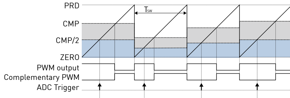
Fig. 4.8: Midpoint sampling for sawtooth carrier, the sampling point is continuously adjusted to be in the middle of the compare value
