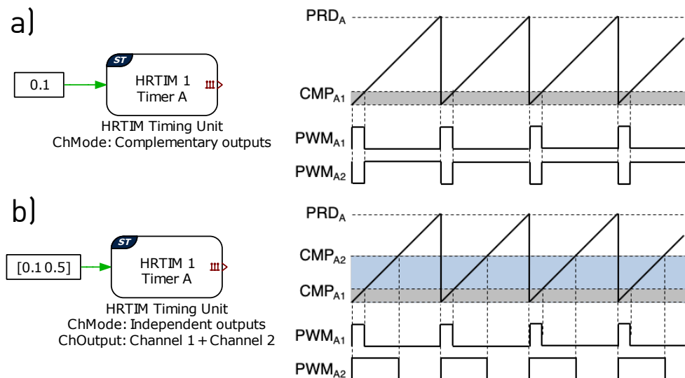
Fig. 4.3: HRTIM timing unit output modes: a) complementary PWM pair, b) two independent PWM outputs
