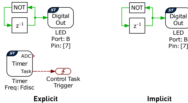
Fig. 2.1: Basic model with control task triggered by Timer
