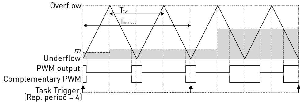
Fig. 2.8: PWM carrier and task interrupts for PWM frequency set to twice the control task frequency
