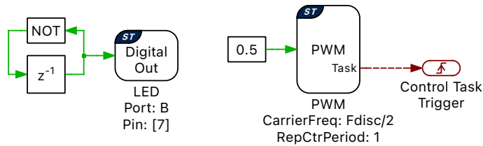
Fig. 2.5: PWM frequency set to half the control task frequency
