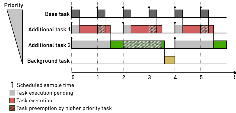
Fig. 2.11: Nested control tasks
