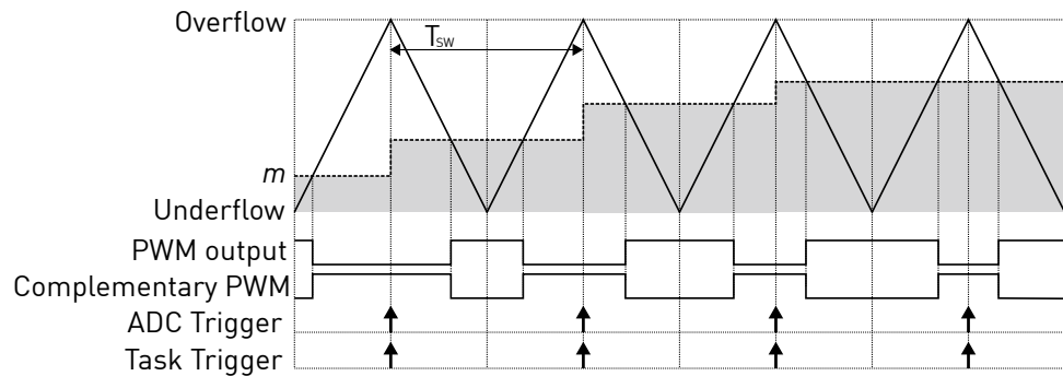
Fig. 4.7: PWM and trigger schemes for symmetric carrier
