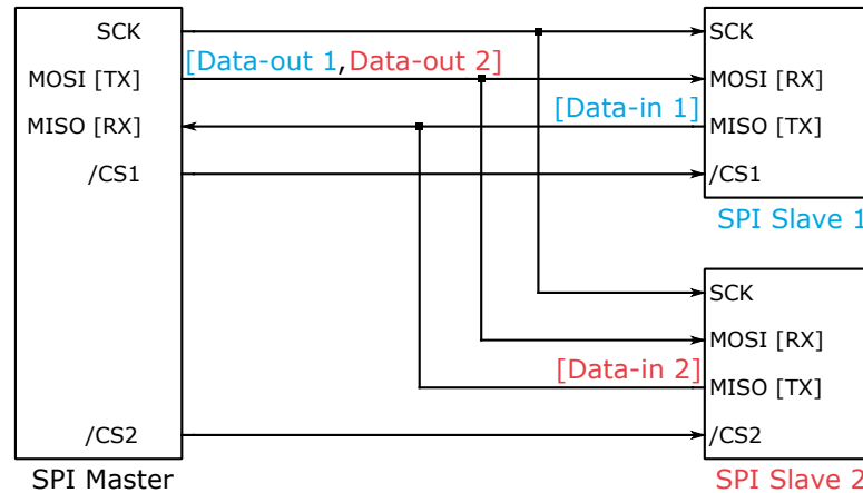
Fig. 4.16: SPI Master with two SPI Slaves
