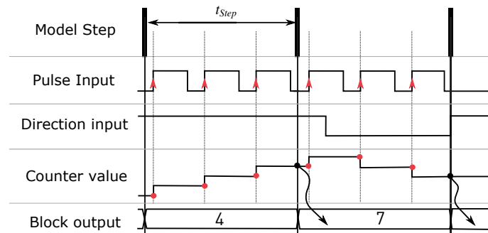
Fig. 4.1: Edge counter value in function of direction signal
