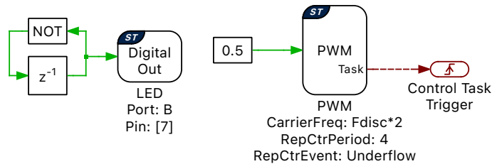
Fig. 2.7: Schematic of PWM frequency set to twice the control task frequency
