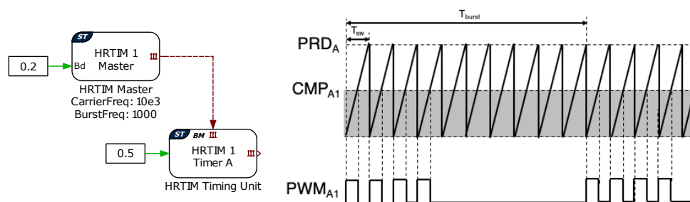
Fig. 4.2: Burst mode controller with a burst mode duty cycle of 0.4.
