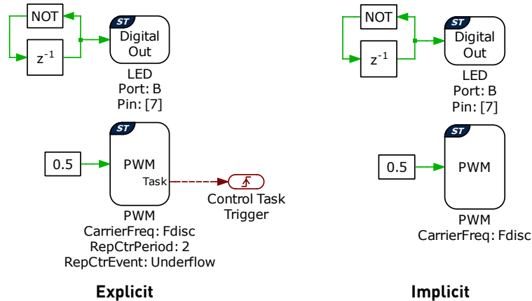
Fig. 2.2: Basic model with control task triggered by PWM
