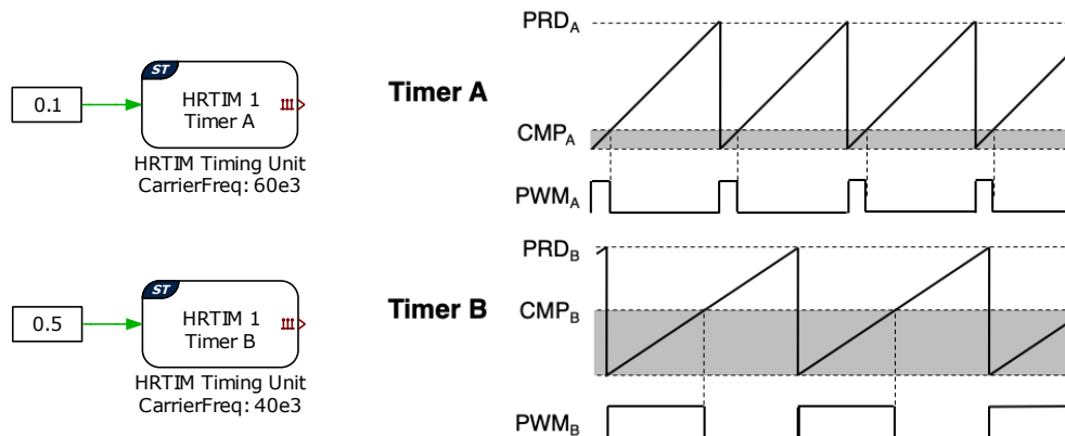
Fig. 4.4: Two independent HRTIM timing units (Self synchronized)
