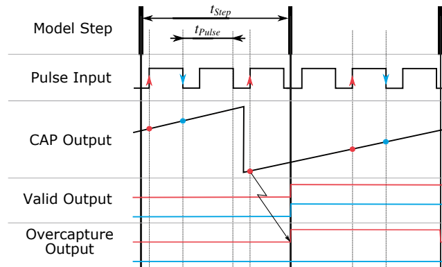
Fig. 4.13: An illustrative example for different capture settings when the Pulse Capture block is used with individual channels (channel 1 in red, channel 2 in blue).
