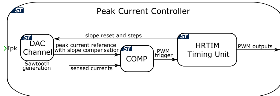
Fig. 4.10: Peak current controller schematic
