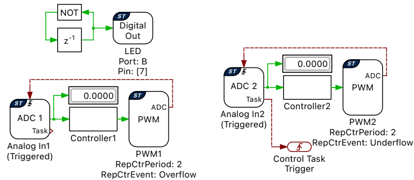
Fig. 2.9: Explicit phase-shifted ADC sampling
