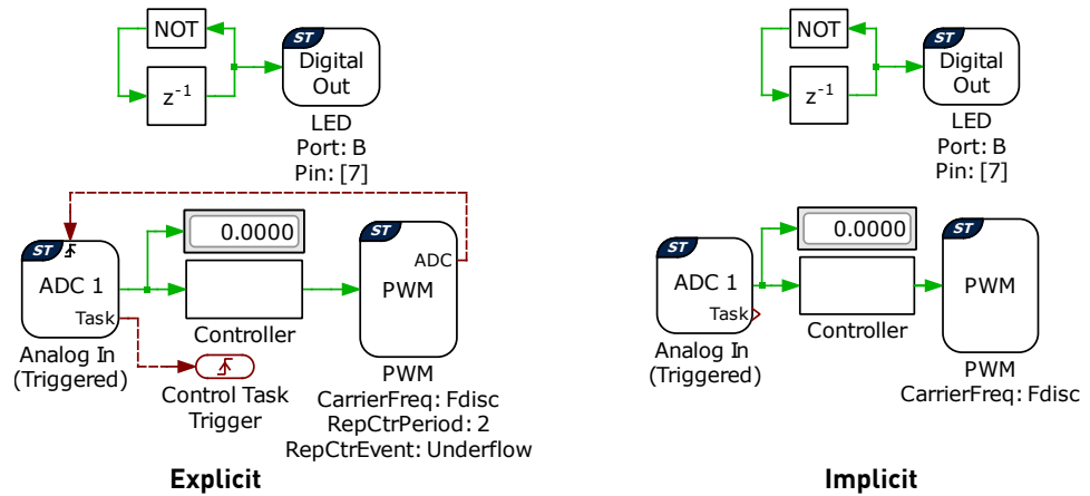
Fig. 2.4: Basic model with control task triggered by PWM via ADC
