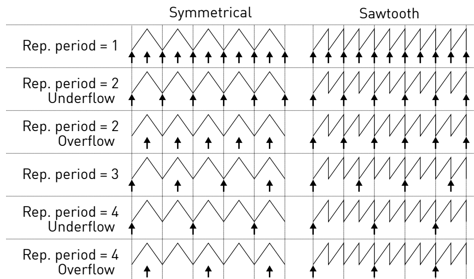
Fig. 4.6: Trigger events based on the repetition counter period
