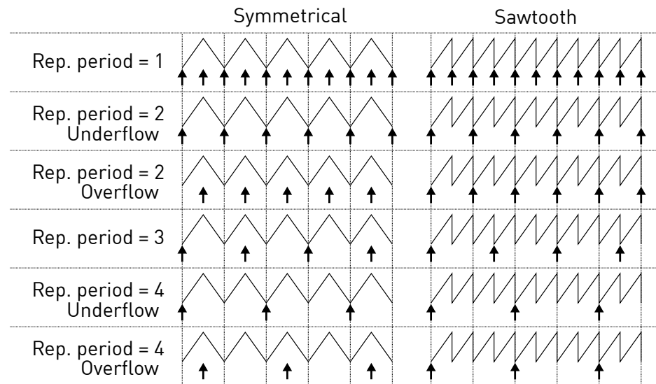
Fig. 4.14: Trigger events based on the repetition counter period
