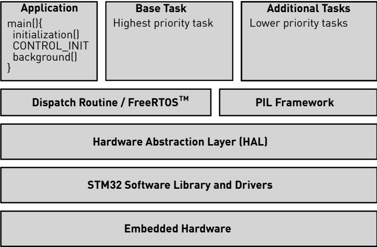
Fig. 2.13: Embedded project architecture
