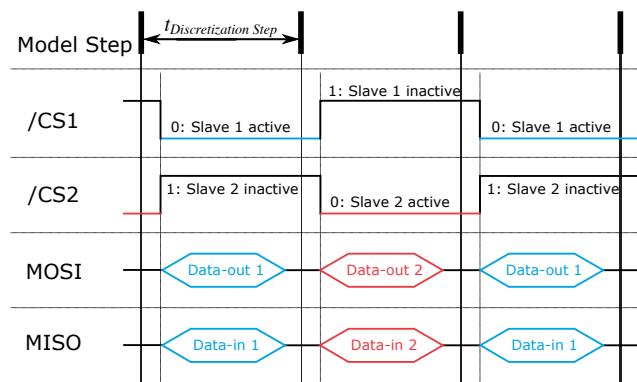
Fig. 4.17: An example of signal exchange between one SPI Master and two SPI Slaves
