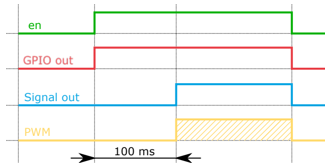
Fig. 4.1 1: Powerstage Protection timing
