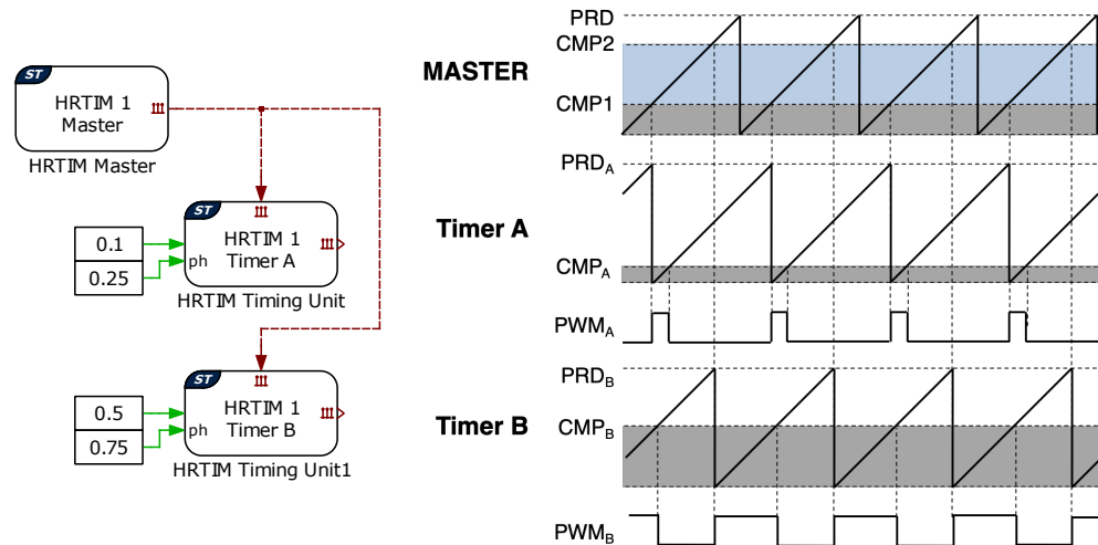
Fig. 4.5: Two HRTIM timing units synchronized to a HRTIM Master block
