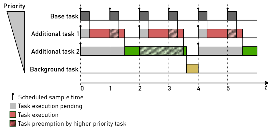
Figure 2.11: Nested control tasks
