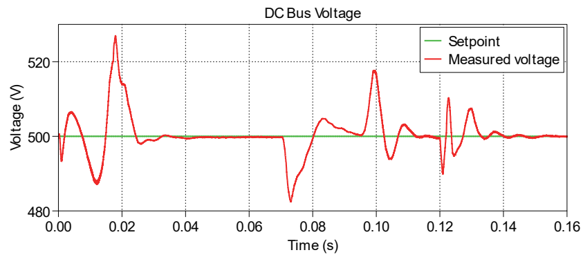
図5: DC電圧
